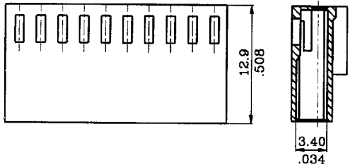
SECTION F-F
