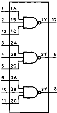
Fig. 1 Logic symbol
