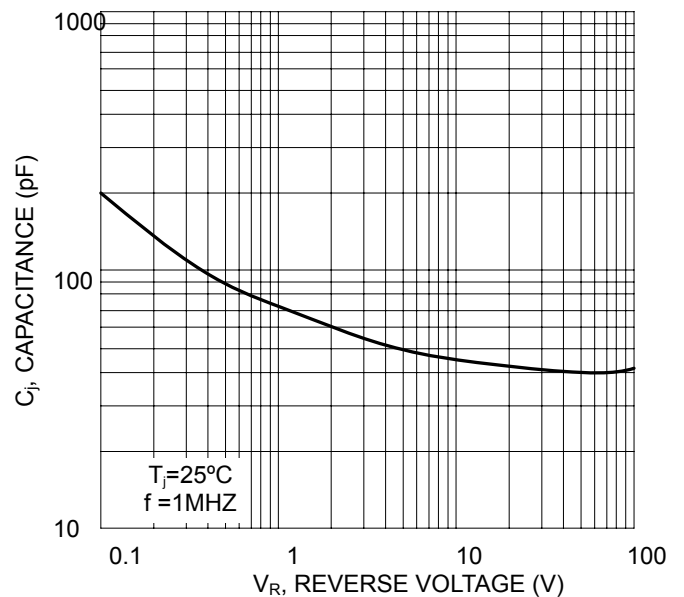
Fig.4 Typ Junction Capacitance per element
