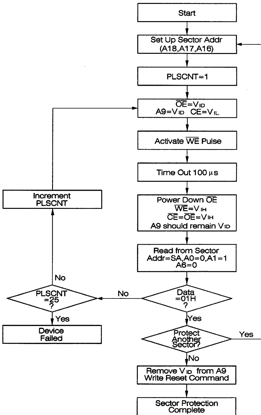
Figure 11 . Sector Protection Algorithm
