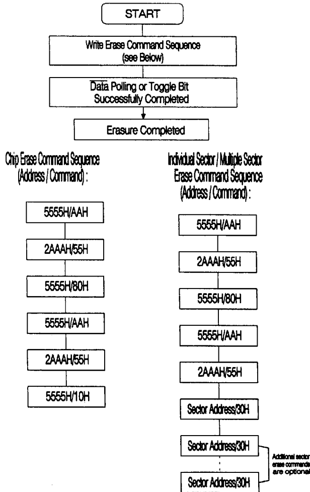
Figure 2. Internal Erase Algorithm
