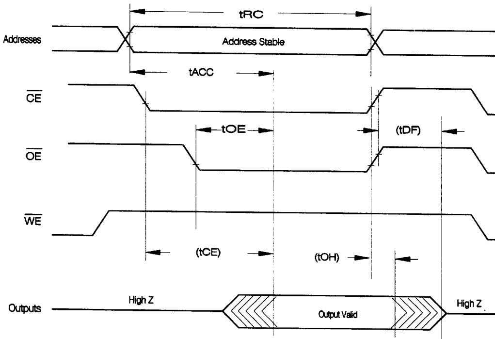
Figure 6. AC Waveforms for Read Operations
