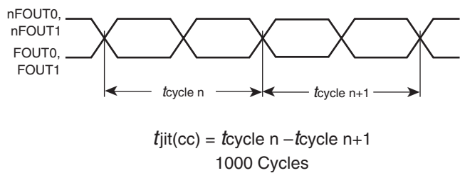
Cycle-to-Cycle Jitter
