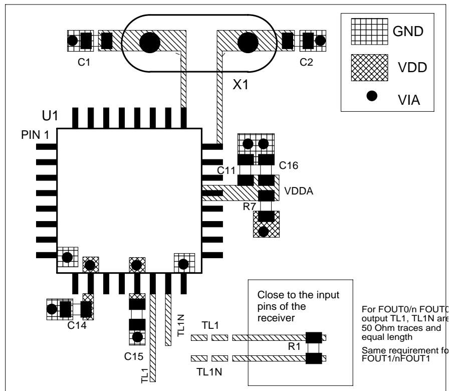
FIGURE 6B. PCB BOARD LAYOUT FOR ICS8442
