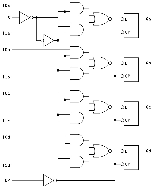
FIGURE 3. Logic diagram.
