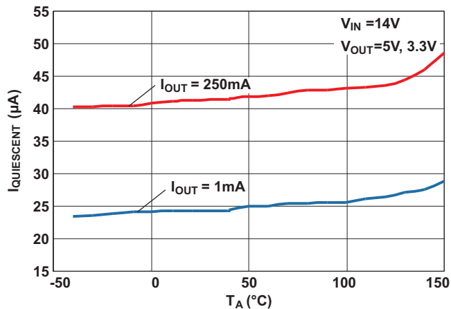
QUIESCENT CURRENT vs AMBIENT AIR TEMPERATURE
