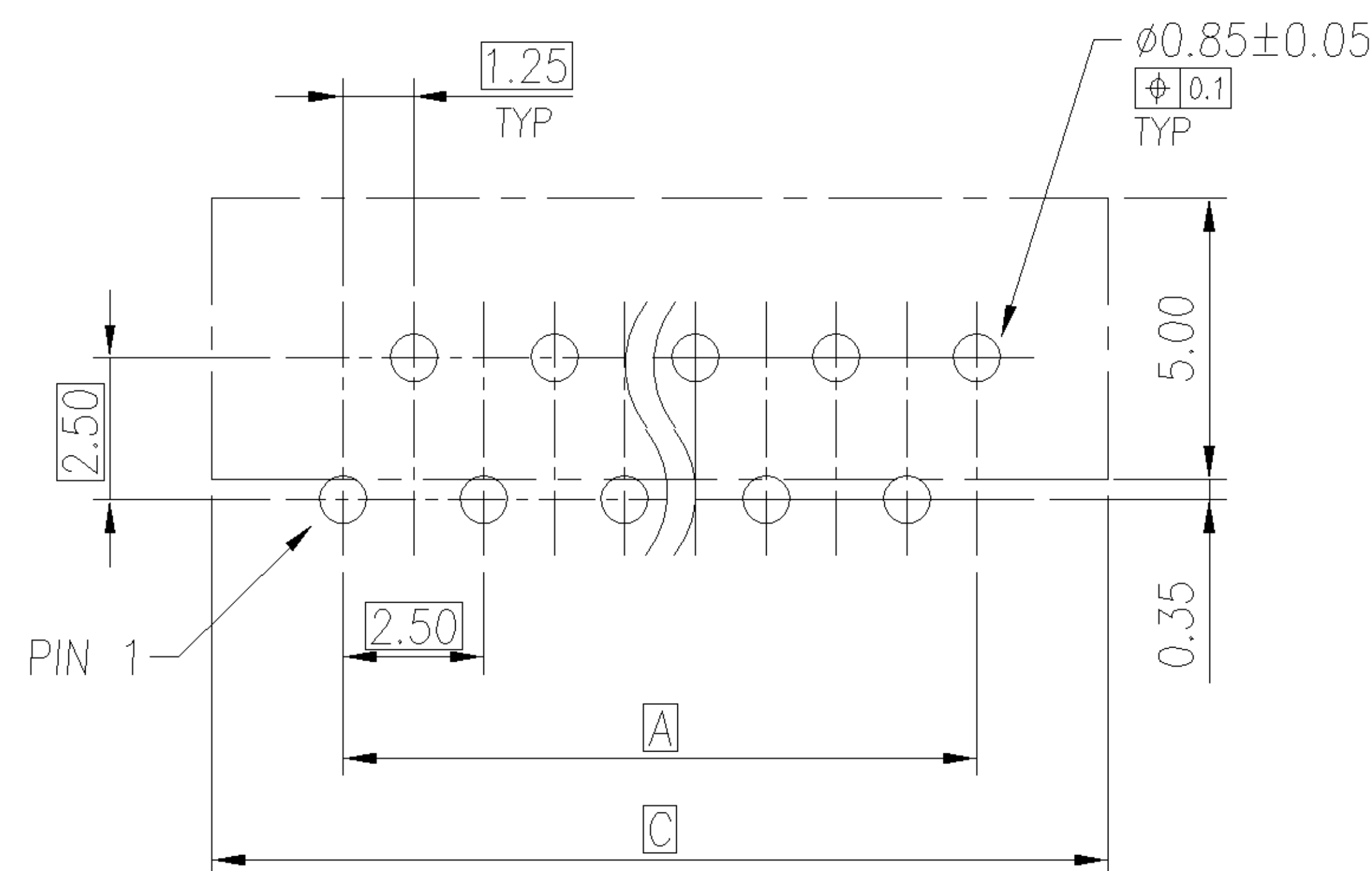
RECOMMENDED PCB LAYOUT PCB TOLERANCE: ±0.05
