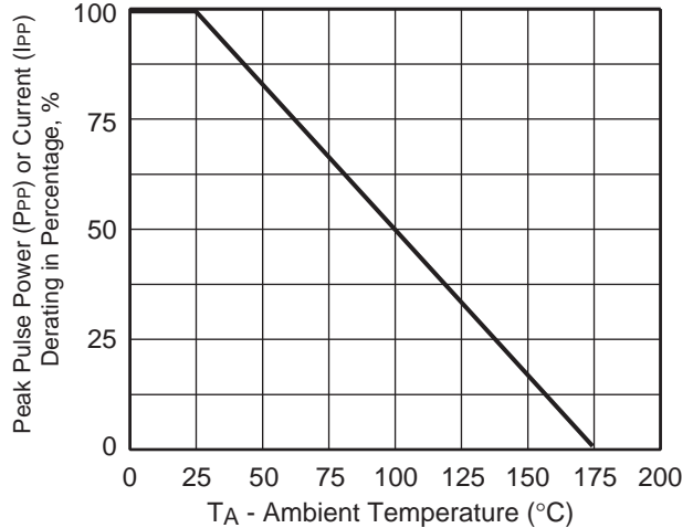
Fig. 2 – Pulse Power Derating Curve
