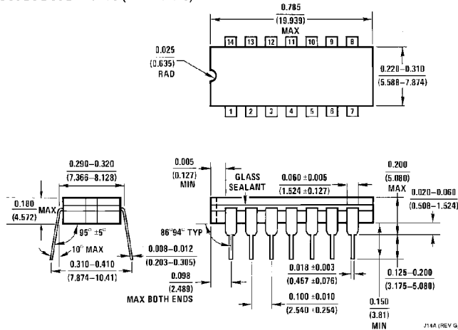
Dual-In-Line Package (J) Order Number MM54HCT34J or MM74HCT34J NS Package J14A
