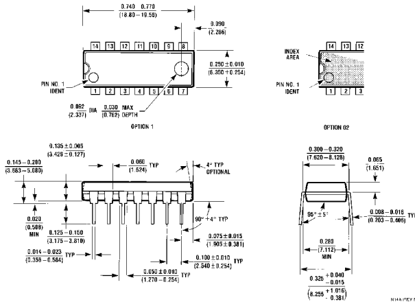
Dual-In-Line Package (N) Order Number MM74HCT34N NS Package N14A
