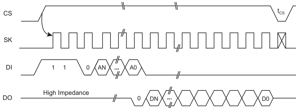
Figure 5-2. Read Timing
