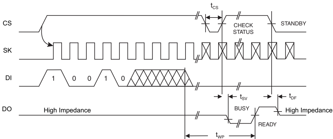
Figure 5-8. ERAL Timing
