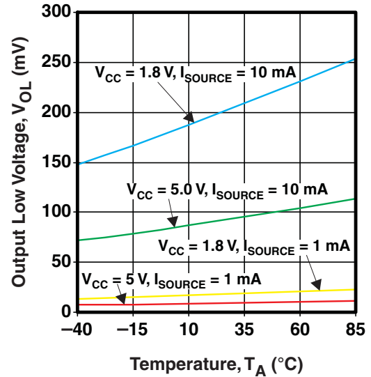
Figure 8. I/O Low Voltage vs Temperature
