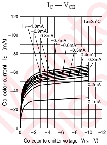
Characteristics charts of UNR6110
