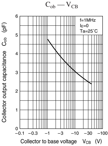
Characteristics charts of UNR6110
