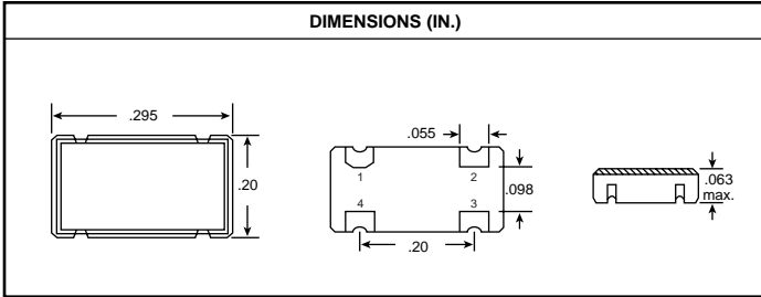
DIMENSIONS (IN.)
