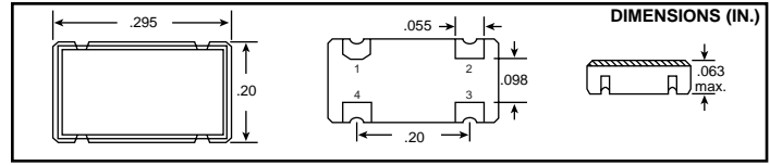
DIMENSIONS (IN.)
