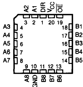
SN54ALS640B, SN54AS640... FK PACKAGE (TOP VIEW)
