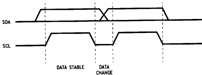
FIGURE 1. Data Validity
