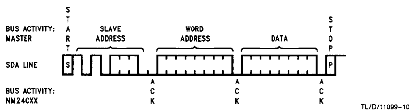
FIGURE 5. Byte Write
