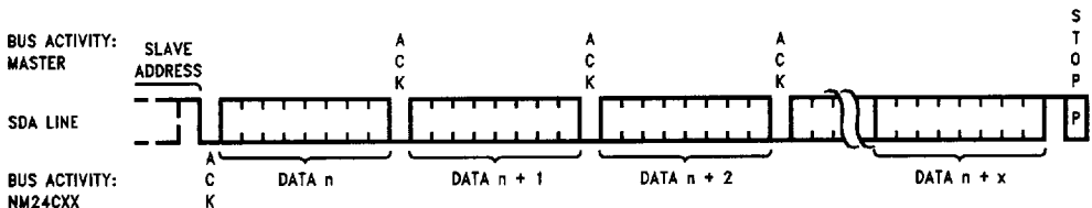
FIGURE 9. Sequential Read
