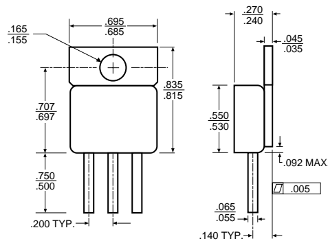
MECHANICAL OUTLINE
