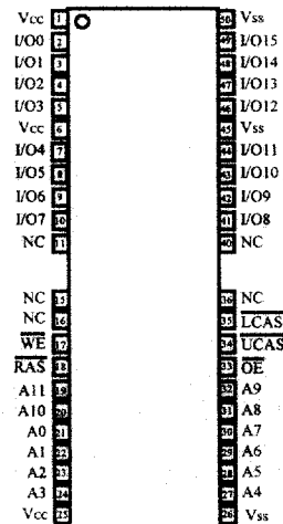
44(50) TSOP II
