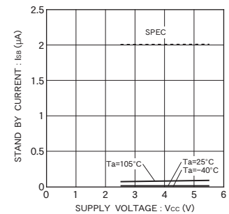
Fig. 13 Consumption current at standby action I_{sb}
