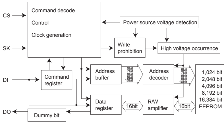
Fig. 27 Block diagram
