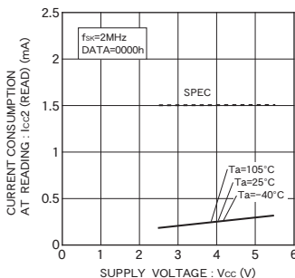
Fig. 11 Consumption current at READ action I_{cc2} (READ, f_{sk}=2MHz )
