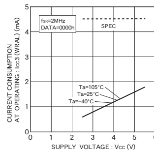
Fig. 12 Consumption current at WRAL action I_{cc3} (WRAL, f_{sk}=2MHz )
