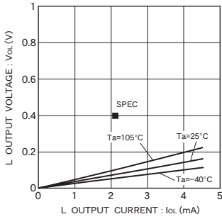
Fig. 5 L output voltage V_{OL-I_{OL}} ( V_{CC}=4.0V )
