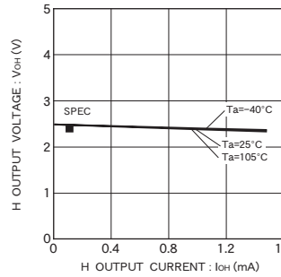
Fig. 6 H output voltage V_{OH-I_{OH}} ( V_{CC}=2.5V )
