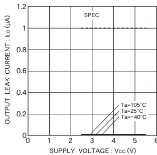
Fig. 9 Output leak current I_{LO} (DO)
