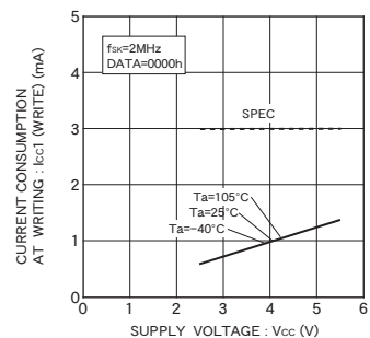
Fig. 10 Current consumption at WRITE action I_{cc1} (WRITE, f_{sk}=2MHz )
