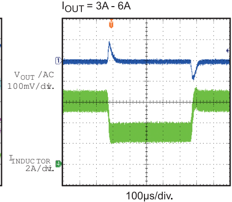
Load Transient Response I_{OUT} = 3A - 6A
