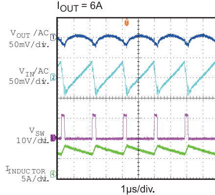
Input / Output Ripple I_{OUT} = 6A
