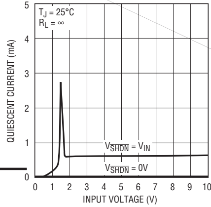
LT1965-1.8 Quiescent Current
