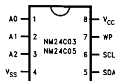
TSSOP Package (MT8)
