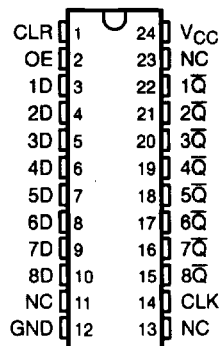
SN74ALS577A . . . DW OR NT PACKAGE (TOP VIEW)
