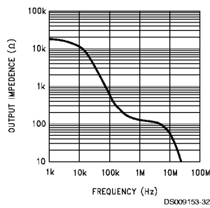
Output Resistance Open-Loop
