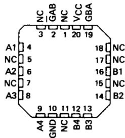
SN54LS242, SN54LS243 . . . FK PACKAGE (TOP VIEW)
