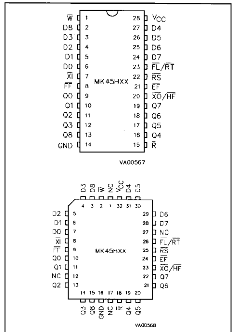
Figure 1. Pin Connections
