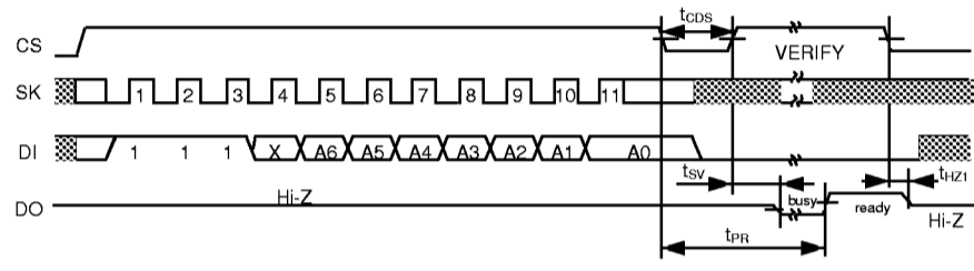
Figure 11 ERASE Timing (S-93C56A)
