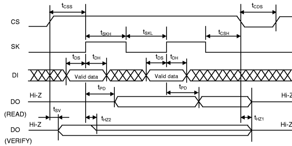
Figure 3 Read Timing
