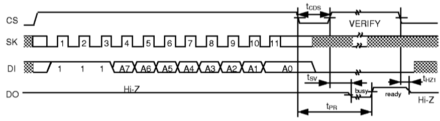
Figure 12 ERASE Timing (S-93C66A)
