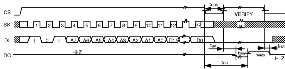
Figure 9 WRITE Timing (S-93C66A)
