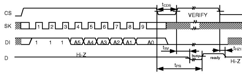
Figure 10 ERASE Timing (S-93C46A)
