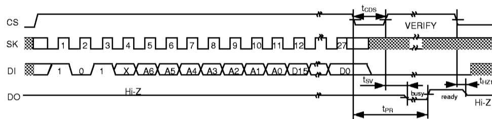
Figure 8 WRITE Timing (S-93C56A)
