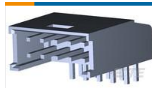
TE Part #284124-1 2X5P MODU II SHRD HDR,RT ANG, 0.38AU
