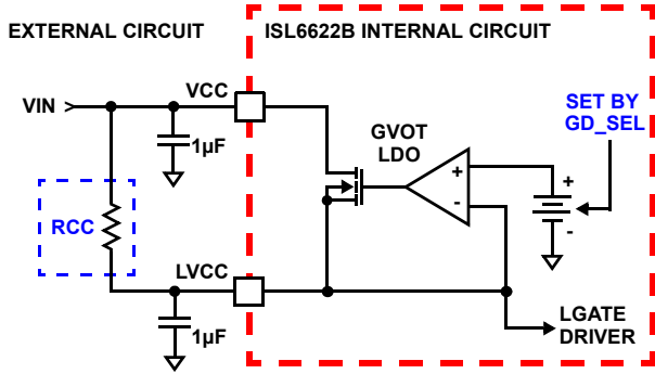
FIGURE 2. GATE VOLTAGE OPTIMIZATION (GVOT) DETAIL
