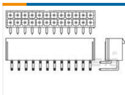
TE Part #1586041-6 6P VAL-U-LOK R/A HDR V2
