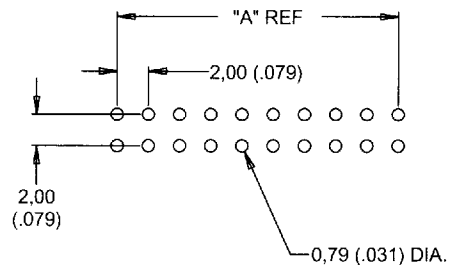
RECOMMENDED PCB HOLE PATTERN
