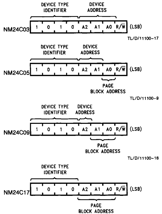
FIGURE 4. Slave Addresses
