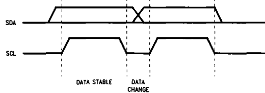
FIGURE 1. Data Validity
