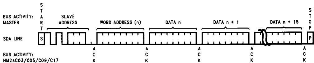
FIGURE 6. Page Write
