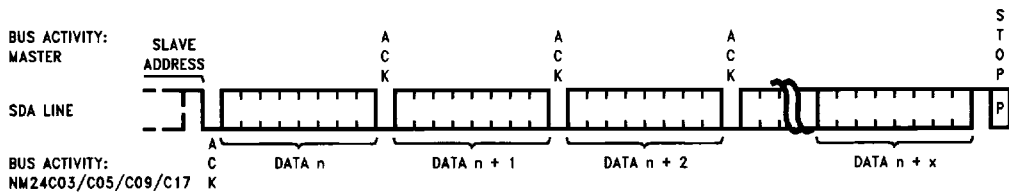
FIGURE 9. Sequential Read
