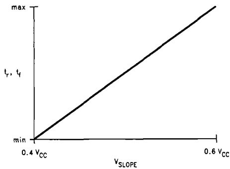
FIGURE 12. Driver Slew Rate vs R_p Pin Control Voltage
