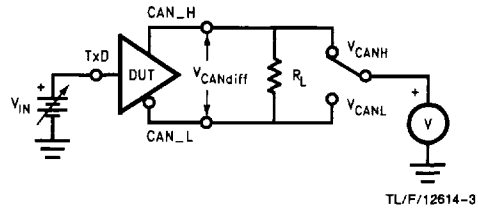
FIGURE 2. Driver V_{CANH} and V_{CANL} Dominant and Recessive
