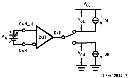
FIGURE 5. Receiver V_{OL}/I_{OL} and V_{OH}/I_{OH}
