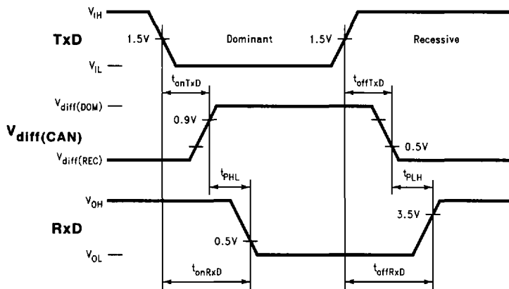
FIGURE 9. Propagation Delays
