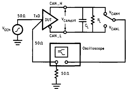
FIGURE 6. Driver Differential Propagation Delay Test Circuit
