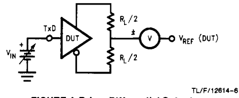
FIGURE 4. Driver Differential Output Voltage Balance ( V_{BAL} )
