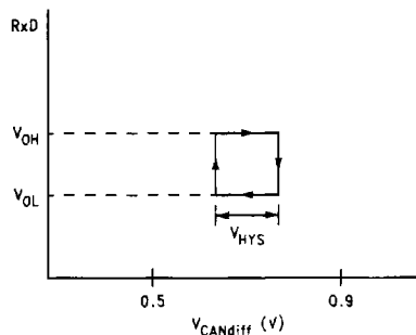
FIGURE 13. Hysteresis
