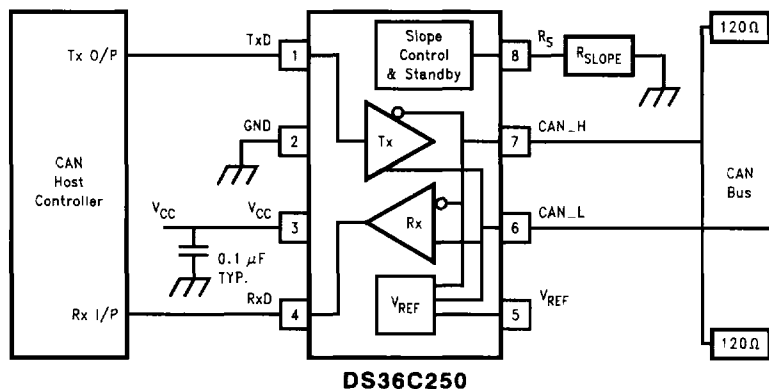
Typical Application with Host Control
