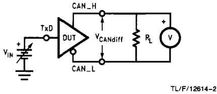
FIGURE 1. Driver V_{CANDiff} Dominant and Recessive
