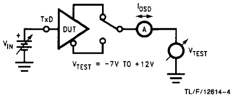
FIGURE 3. Driver I_{OSD}
