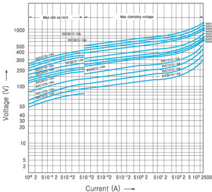
10A(SVC 820D-10A to SVC 471D-10A)
