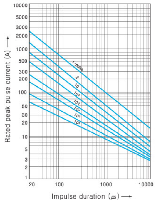
10A(SVC 820D-10A to SVC 471D-10A)
