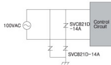
Vending Machine
