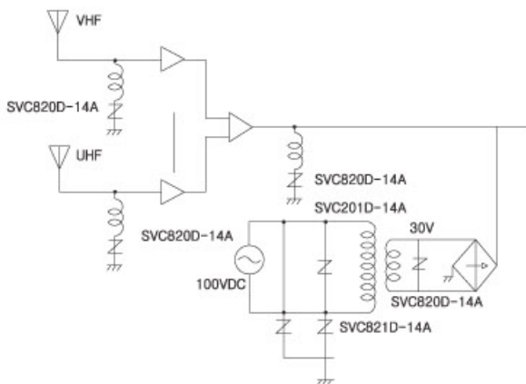
TV Booster
