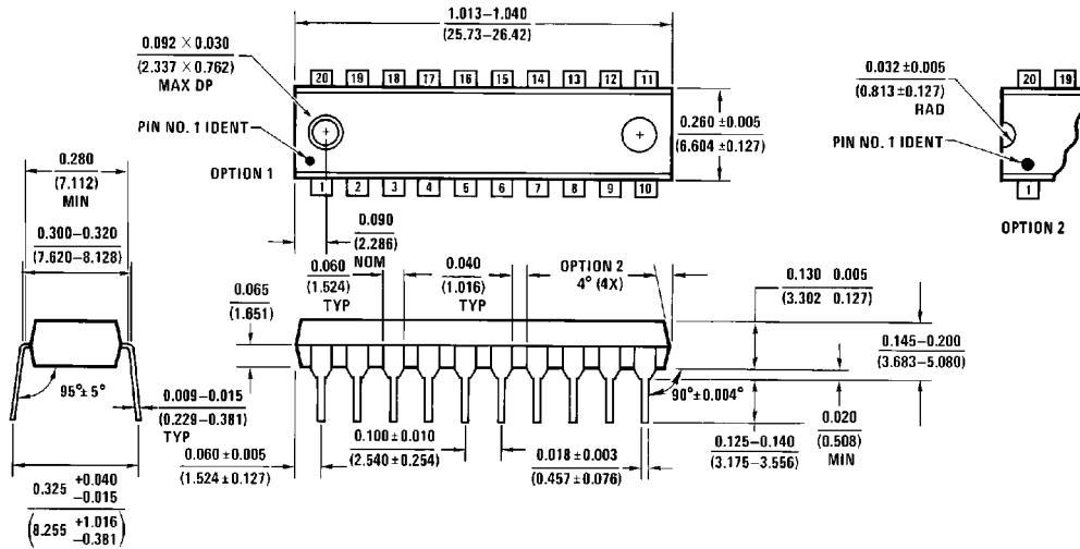
20-Lead Plastic Dual-In-Line Package (P) NS Package Number N20A
