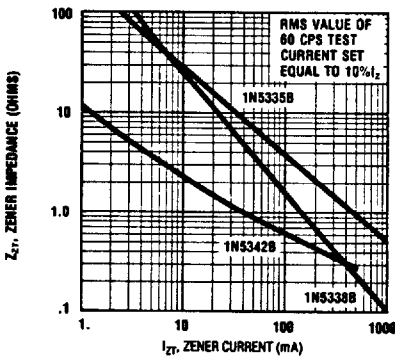
TYPICAL ZENER IMPEDANCE VS. ZENER CURRENT FOR TYPES SHOWN
