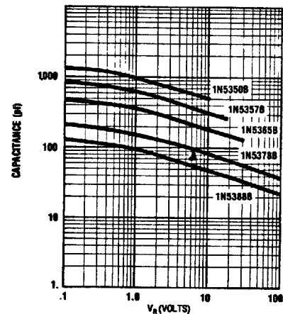
TYPICAL CAPACITANCE vs REVERSE VOLTAGE FOR 5 WATT ZENERS
