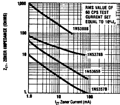
TYPICAL ZENER IMPEDANCE VS. ZENER CURRENT FOR TYPES SHOWN
