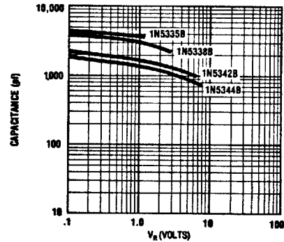
TYPICAL CAPACITANCE vs REVERSE VOLTAGE FOR 5 WATT ZENERS
