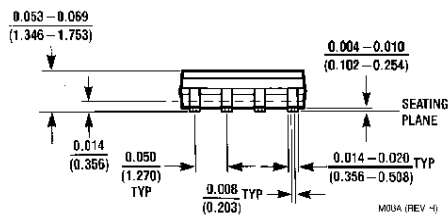
Molded Package, Small Outline, 0.15 Wide, 8-Lead (M8) NS Package Number M08A
