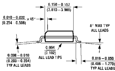
Molded Package, Small Outline, 0.15 Wide, 8-Lead (M8) NS Package Number M08A
