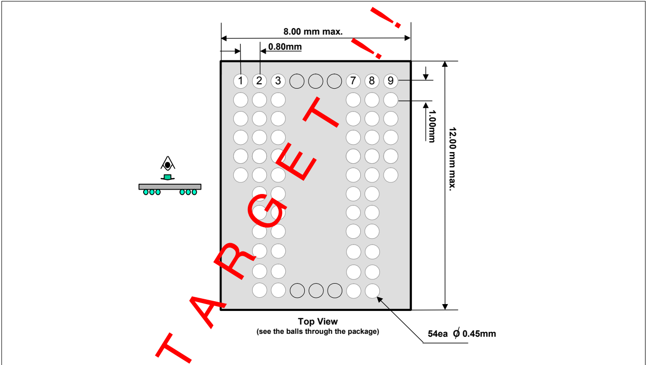
Figure 51 P-TFBGA-60 (Plastic Thin Fine-Pitch Ball Grid Array Package)
