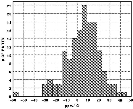
Figure 2. Typical Output Voltage Temperature Drift Distribution
