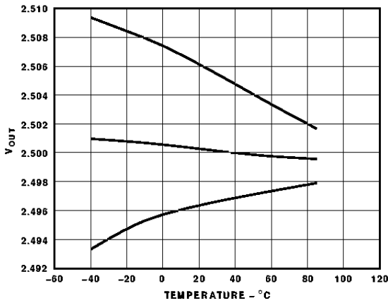
Figure 4. Typical Temperature Drift Characteristic Curves
