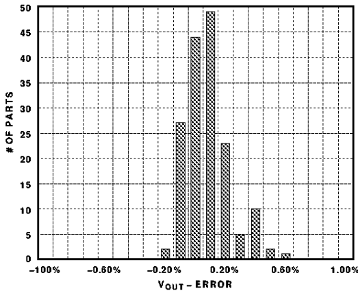
Figure 3. Typical Output Voltage Error Distribution
