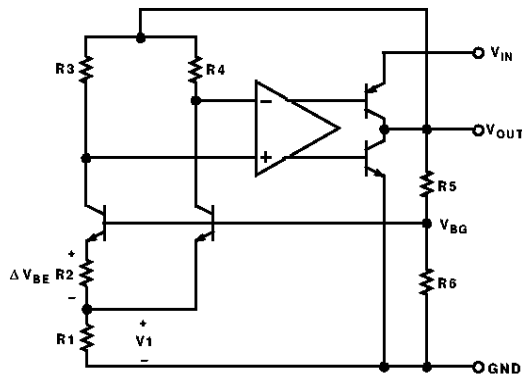
Figure 8. Simplified Schematic
