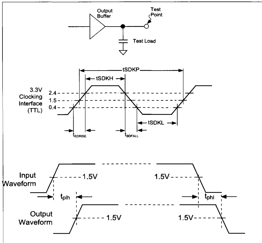
Figure 1. Clock Waveforms
