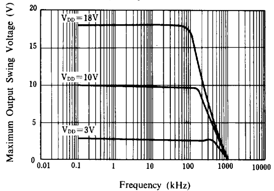
Maximum Output Swing Voltage vs. Frequency
