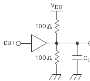
TEST CIRCUIT B OR EQUIVALENT (DEVICE TYPES 02 AND 03)
