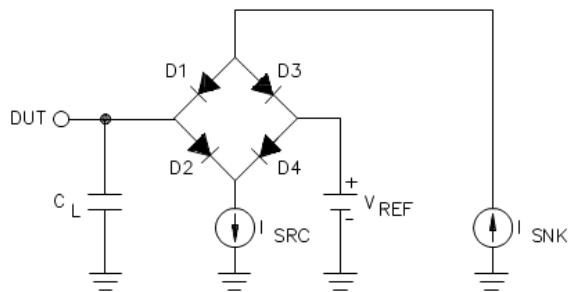
TEST CIRCUIT A OR EQUIVALENT (DEVICE TYPE 01)
