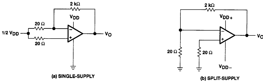
Figure 2. Noise-Test Circuit
