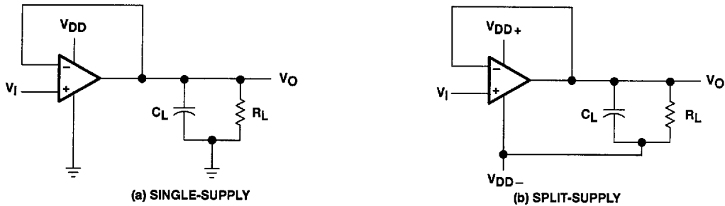
Figure 1. Unity-Gain Amplifier
