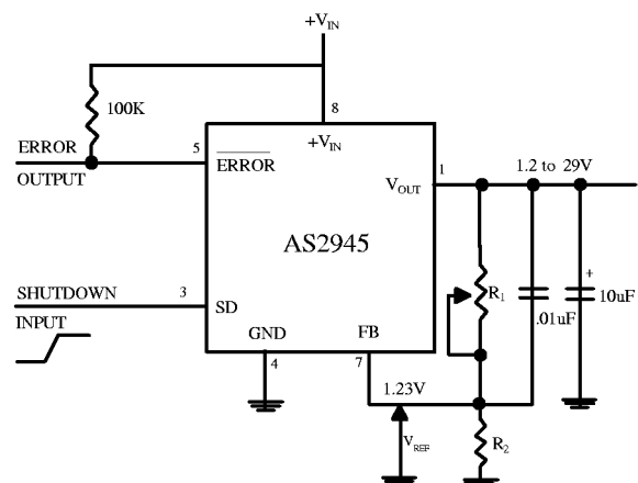
Figure 2. Adjustable Regulator
