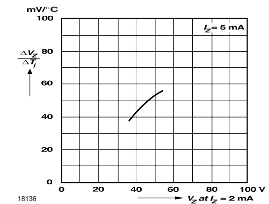
Figure 12. Temperature dependence of Zener voltage versus Zener voltage
