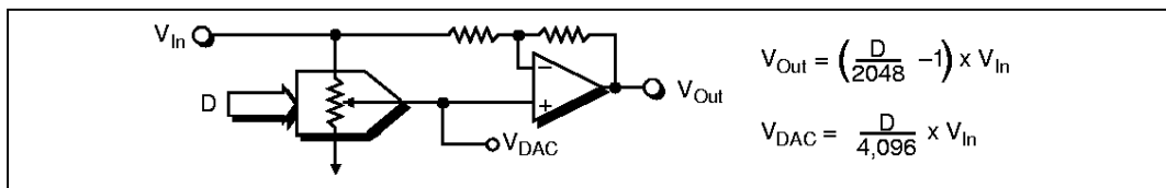
Figure 2. Transfer Function
