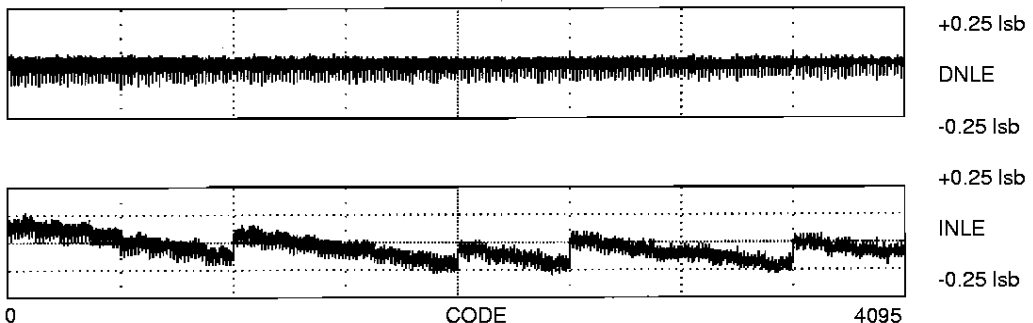
0 CODE 4095 INLE, DNLE Plots
