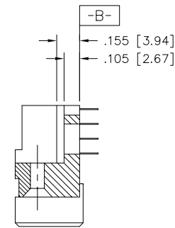
SECTION W-W
