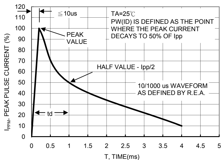
FIG. 7 PULSE WAVEFORM
