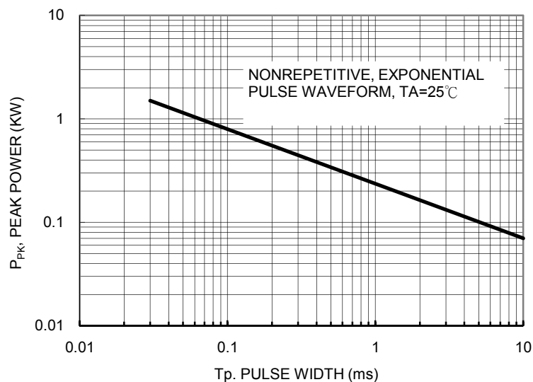
FIG. 6 TYPICAL PULSE RATING CURVE
