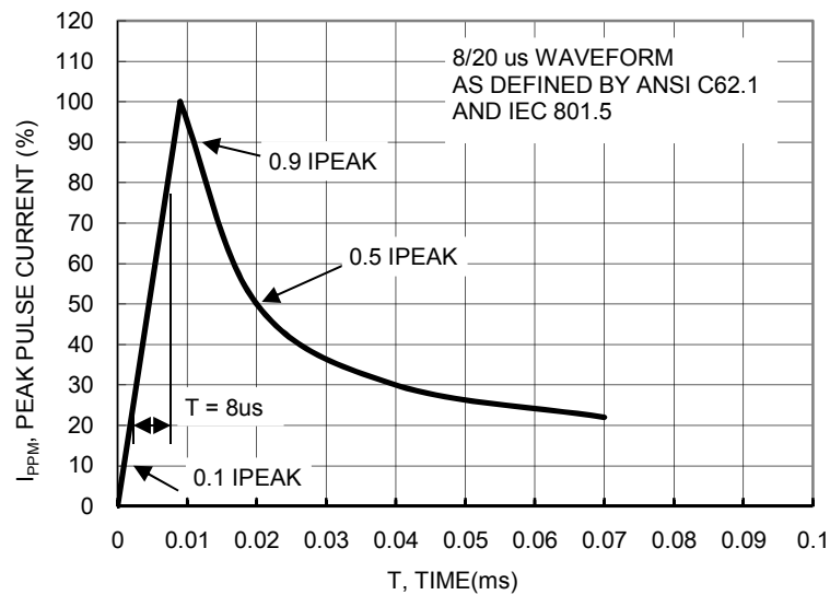
FIG. 8 PULSE WAVEFORM
