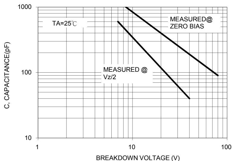
FIG.5 CAPACITANCE CURVE
