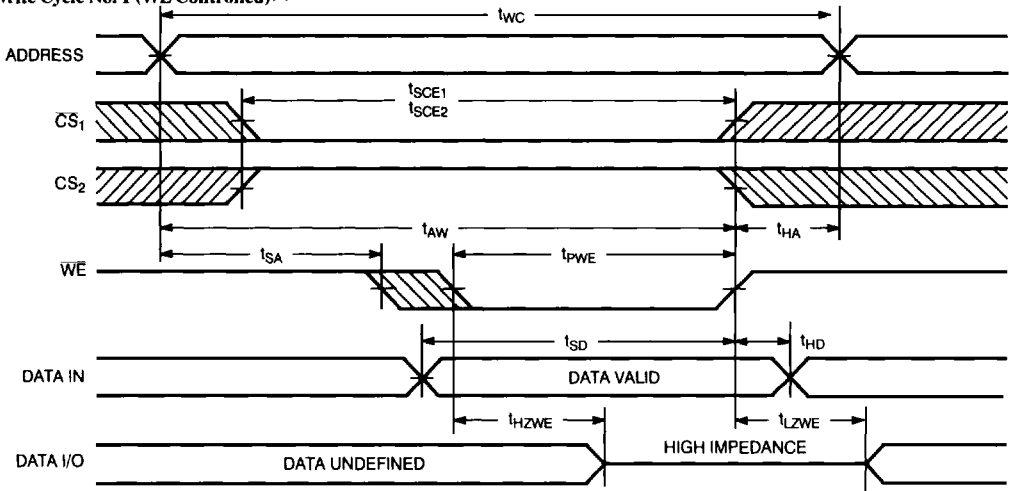
Write Cycle No. 1 ( \overline{WE} Controlled) [7]
