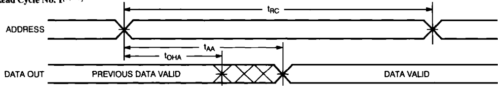
Read Cycle No. 2 [5, 11]
