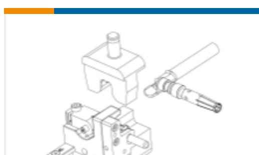
TE Part #2358637-1 DIE SET DIA 6MM-90 T 25MM2
